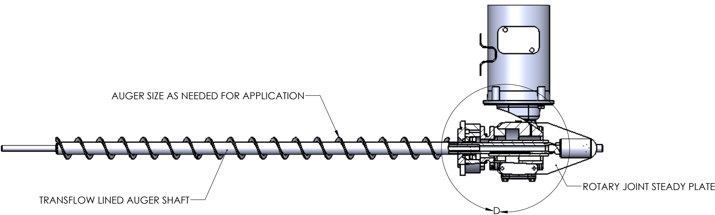
ASSY: AUGER AND DRIVE REMOVED FROM FEEDER
