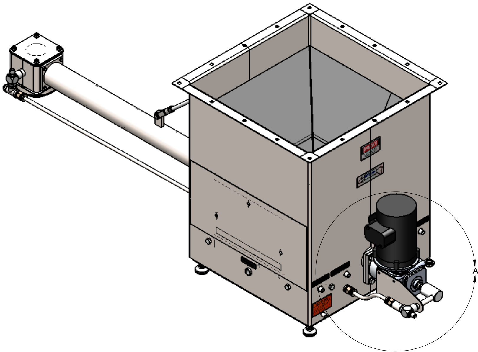
ASSY: TRANSFLOW AUGER ASSY SHOWN WITH MODEL 1 FEEDER ASSEMBLY REF. DRAWING D-20623-01
