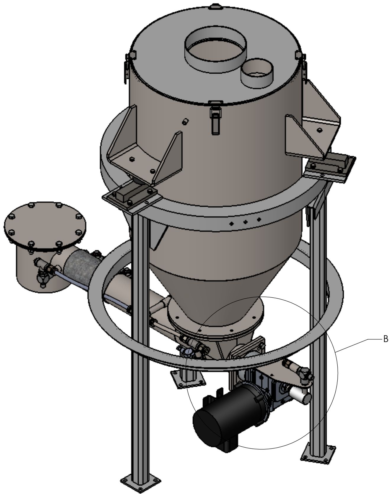
ASSY: TRANSFLOW AUGER ASSY SHOWN WITH MODEL 2 FEEDER ASSEMBLY REF. DRAWING D-20567-03
